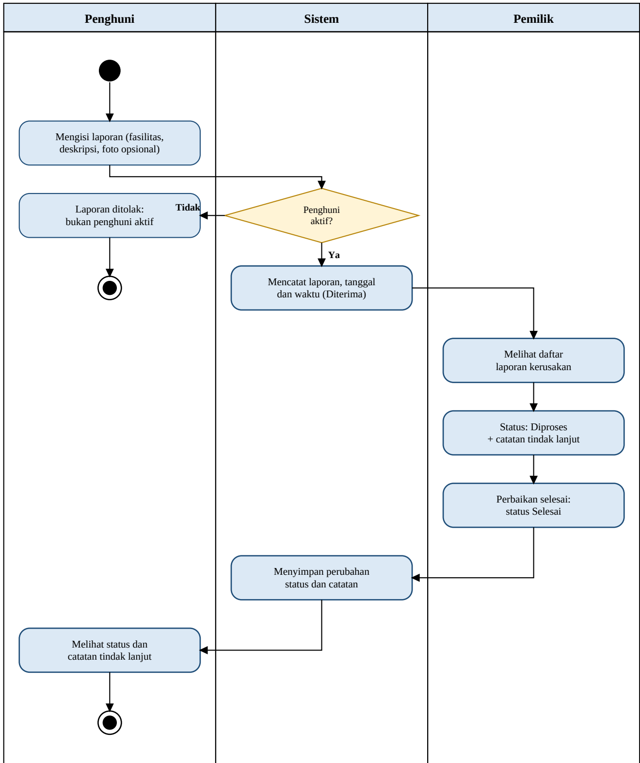
Gambar D.4 Activity Diagram Laporan Kerusakan Fasilitas
