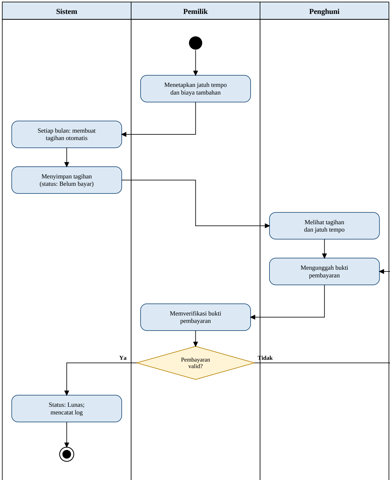
Gambar D.3 Activity Diagram Tagihan Bulanan Otomatis
